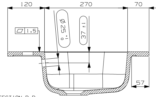
SECTION D-D SCALE 1:5
